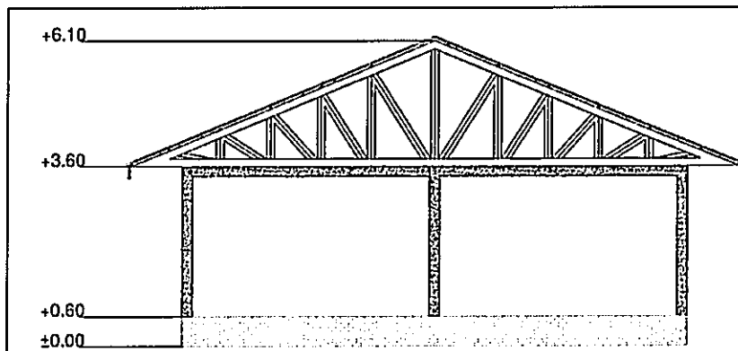
FACADE ARRIERE
